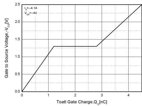
Figure6. Gate Charge
